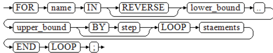
图 10-27 for_loop ::=
