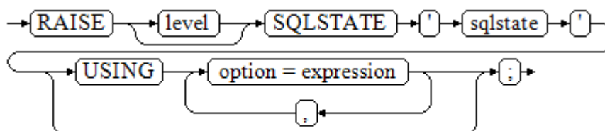
图 10-49 raise_sqlstate::=
