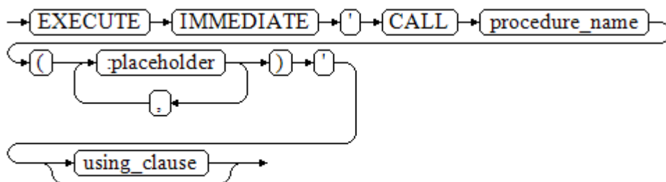
图 10-13 call_procedure::=
