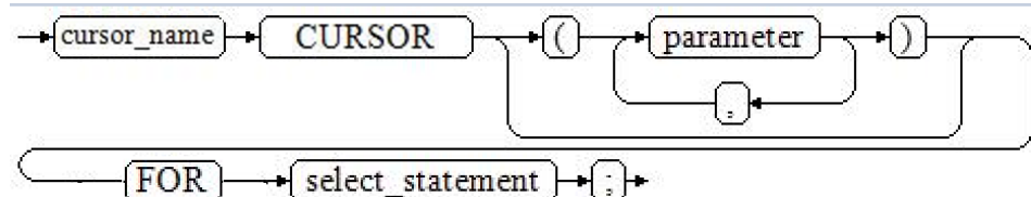
图 10-38 static_cursor_define::=
