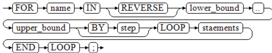
图 10-24 for_loop ::=
