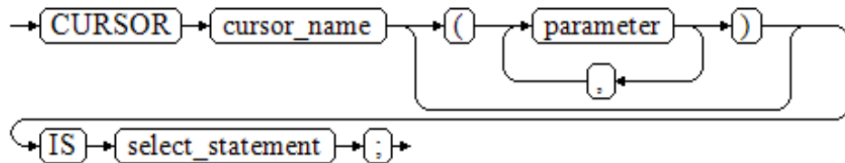
图 10-37 static_cursor_define::=
