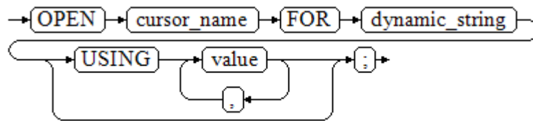
图 10-10 open_for::=
